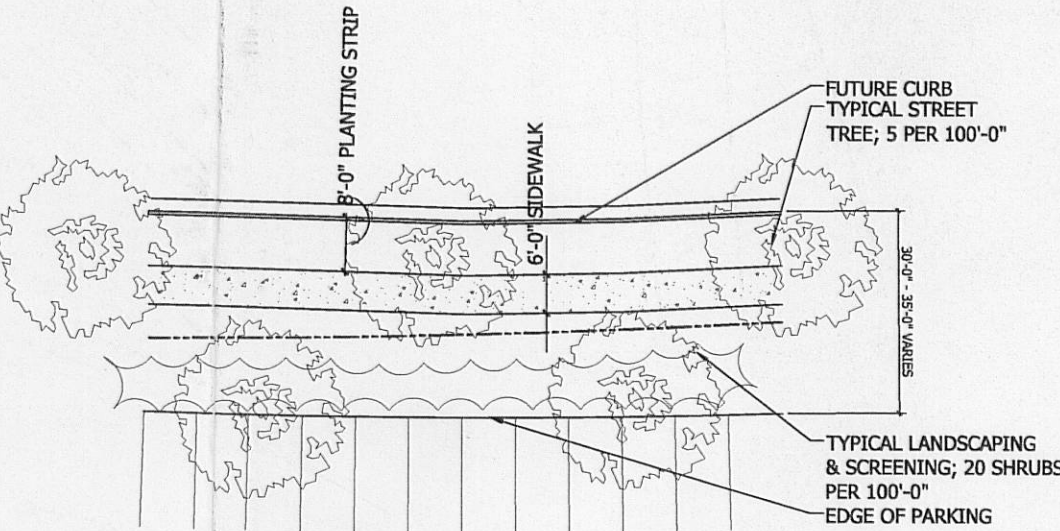
02 TYP. 100' SECTION HARRIS BLVD.
