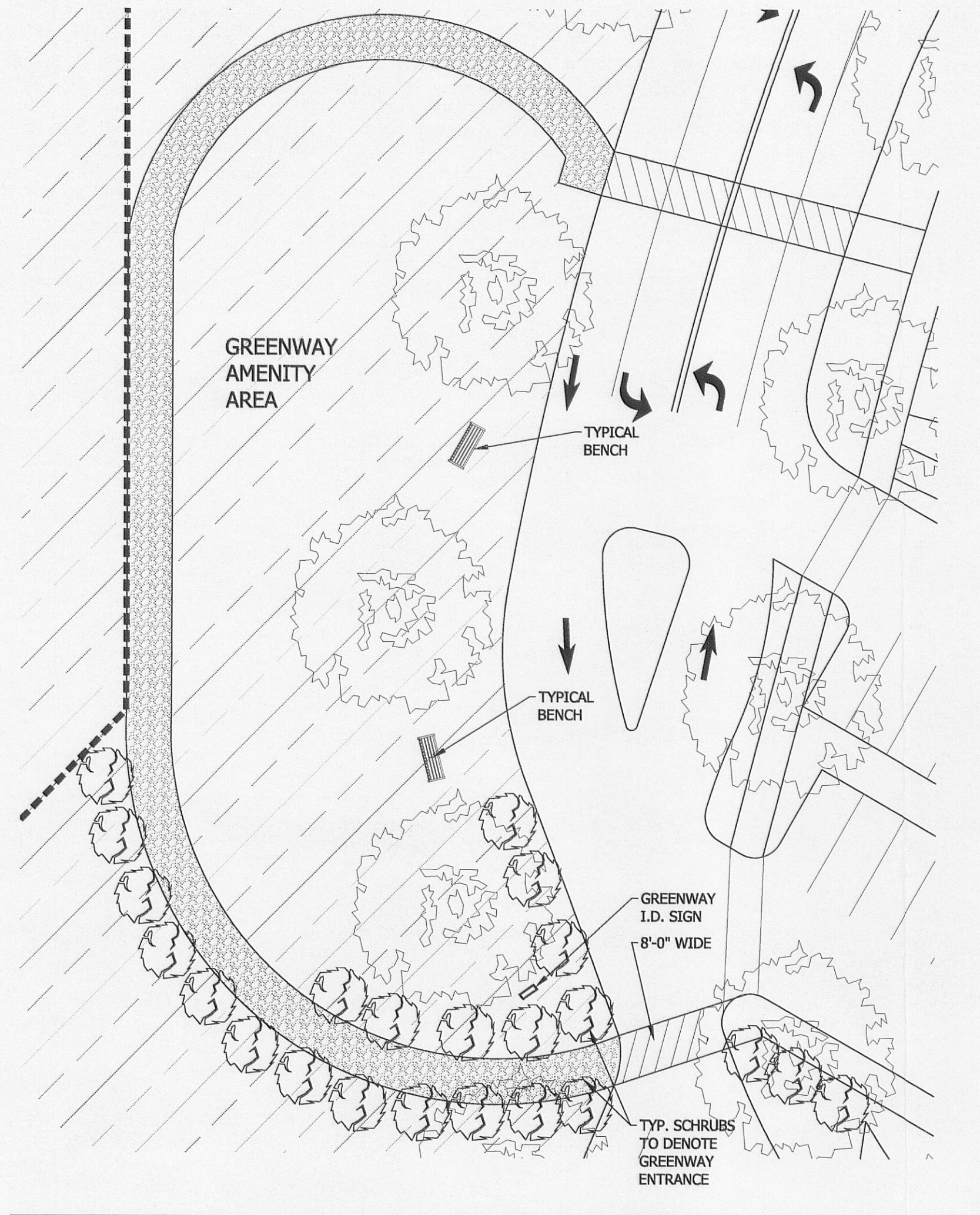
03 ILLUSTRATIVE PLAN - GREENWAY AMENITY AREA 1"=20'-0"
