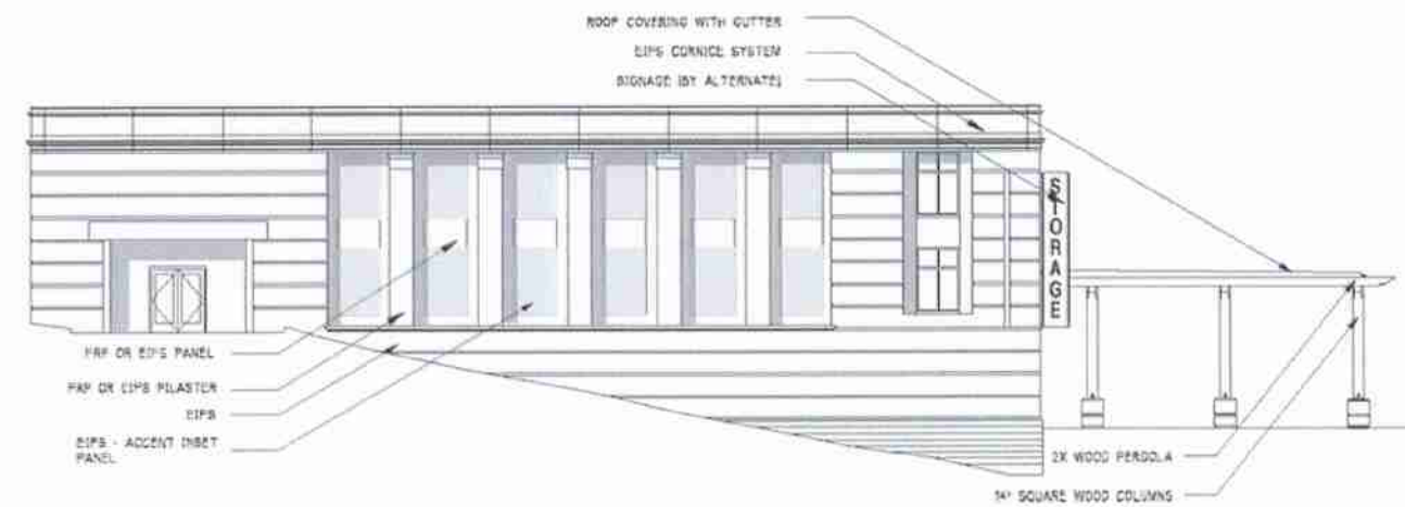
West Elevation
