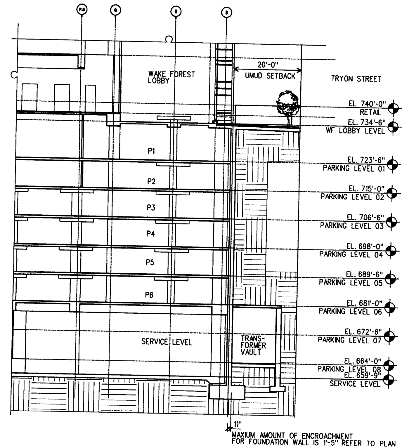
Section \frac{1}{8}'' = 1'-0''
