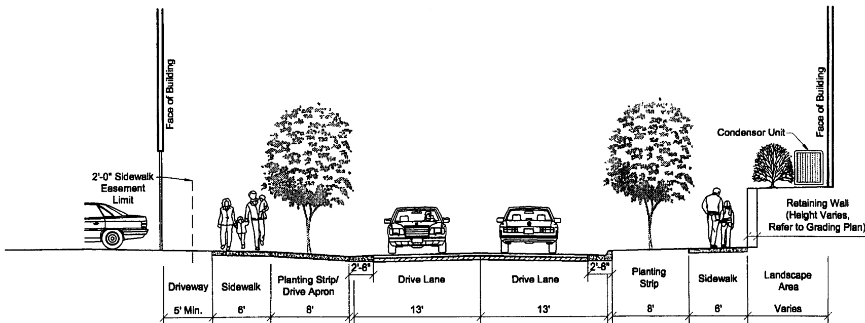
JONES CROSSING ROAD D - D' Cross-Section
