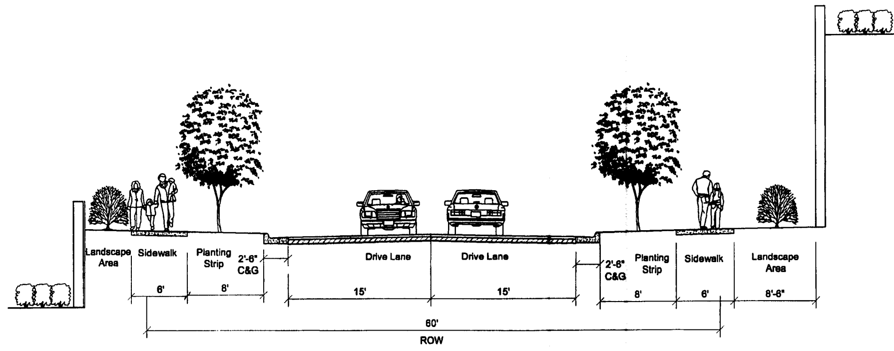
HAWFIELD WAY DRIVE J - J' Cross-Section
