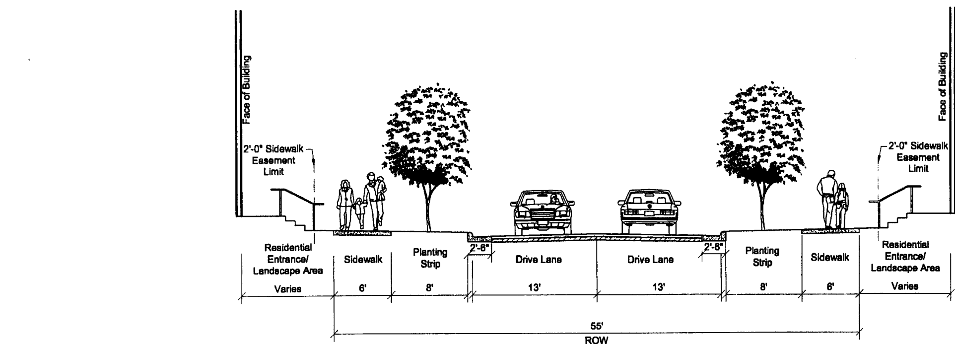
HAWFIELD WAY DRIVE A - A' Cross-Section
