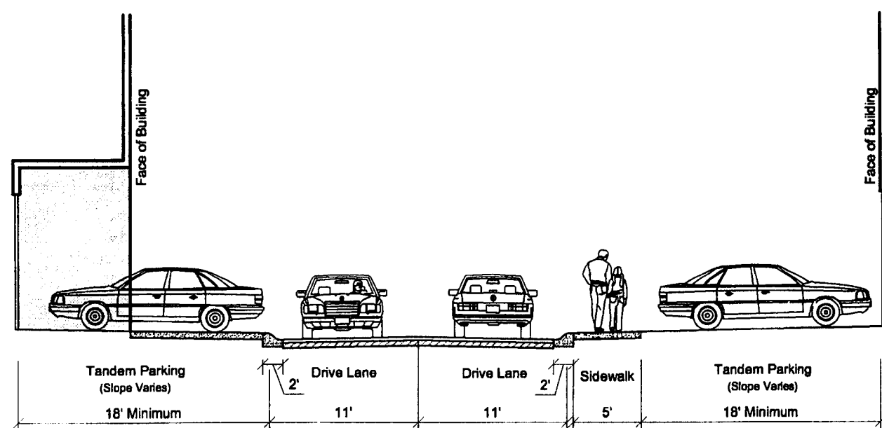
HAWFIELD FARMS ROAD (PRIVATE STREET) E - E' Cross-Section
