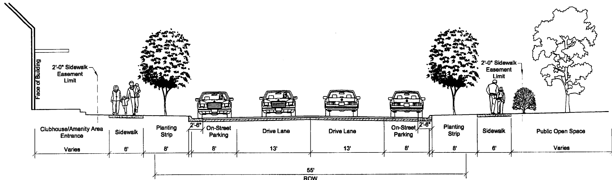
HAWFIELD WAY DRIVE B - B' Cross-Section
