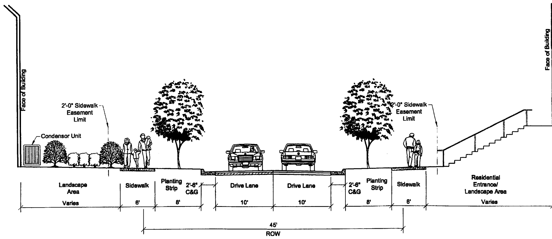
BLAIRBETH STREET C - C' Cross-Section
