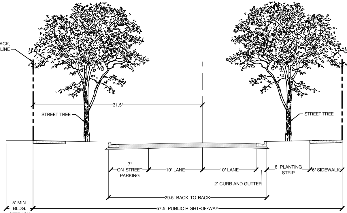
SECTION A-1 (USDG U-03A LOCAL RESIDENTIAL WIDE - MODIFIED)
