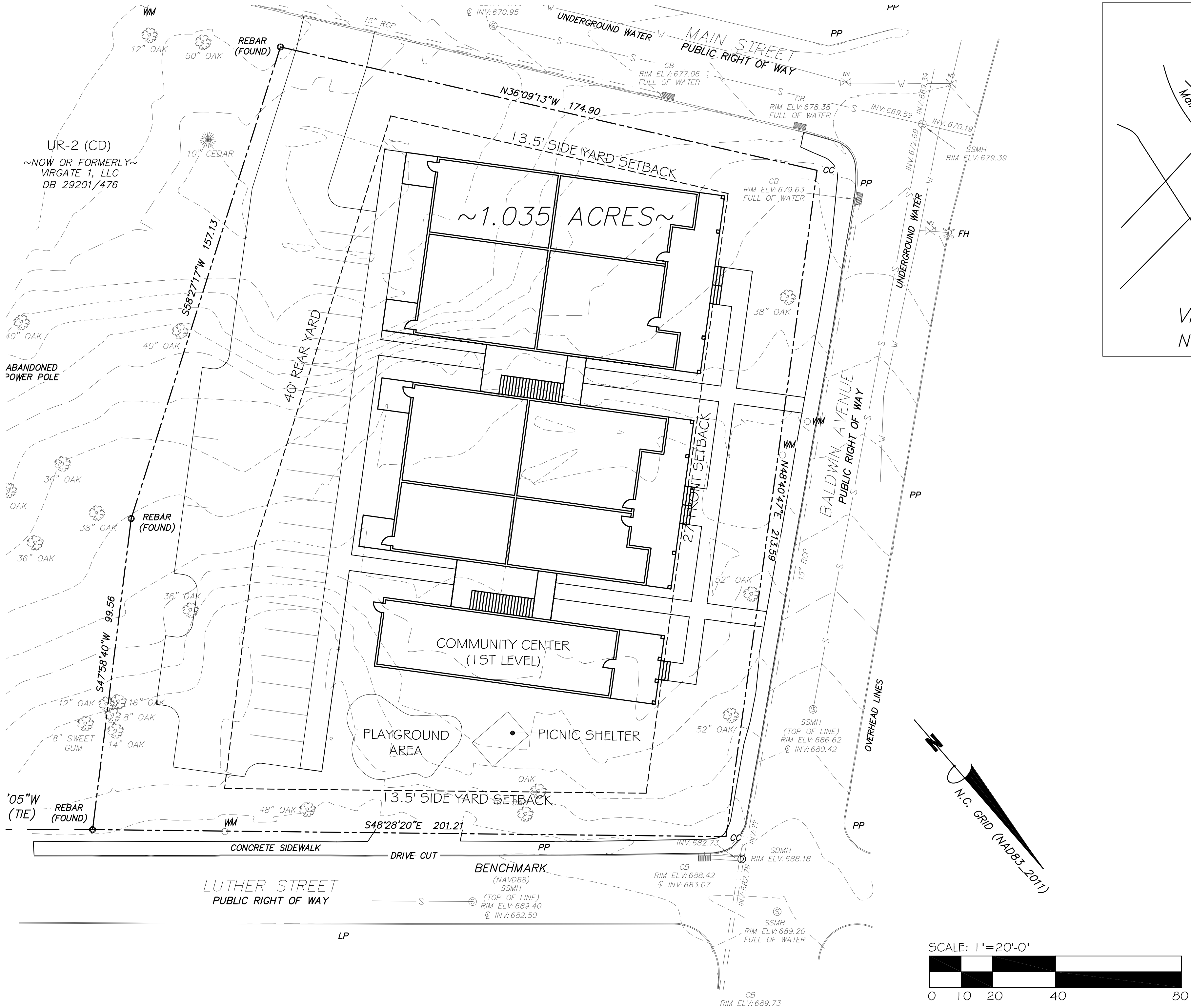
SITE PLAN
