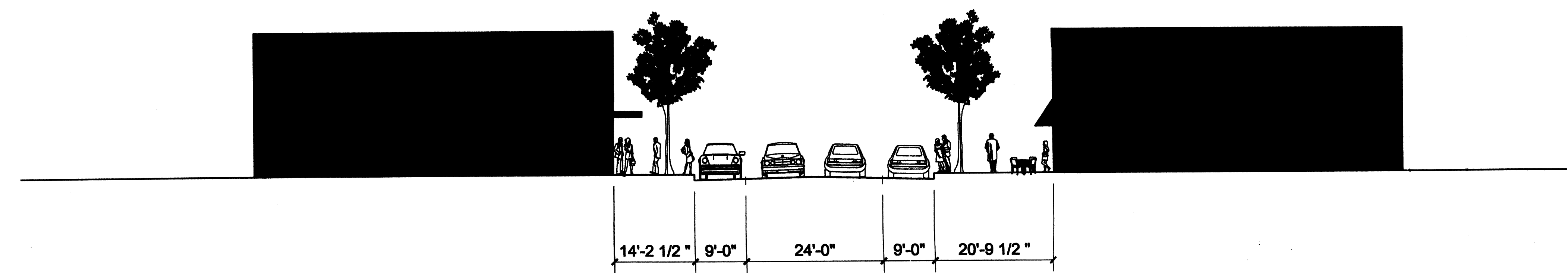
SECTION A
