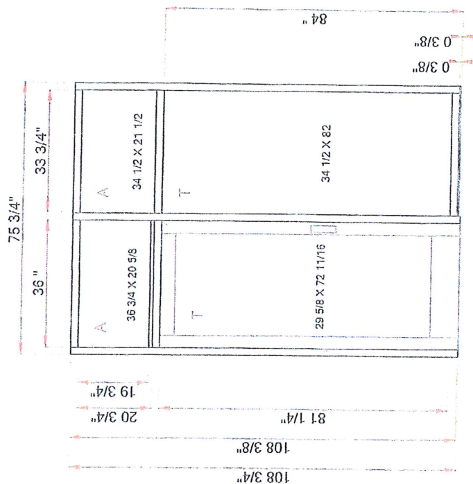
Charlotte Montesori - 002 - Front Left Door.dxf (1 Thus) Frame: (DkBronze) YES 45 TU : Storefront : Screw Spline : Thermal : Inside Glaze
