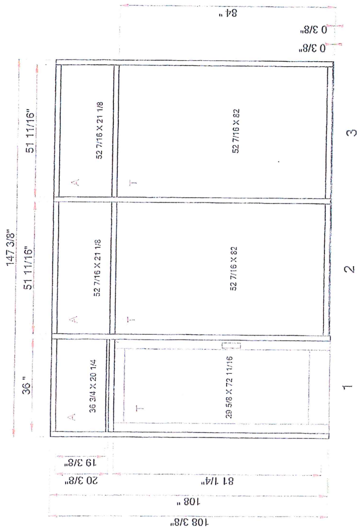
Charlotte Montesori - 001 - New Front Center.dxf (1 Thus) Frame: (DkBronze) YES 45 TU : Storefront : Screw Spline : Thermal : Inside Glaze
