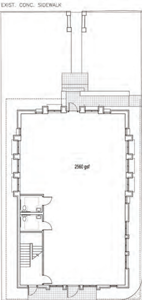
FIRST FLOOR/SITE PLAN
