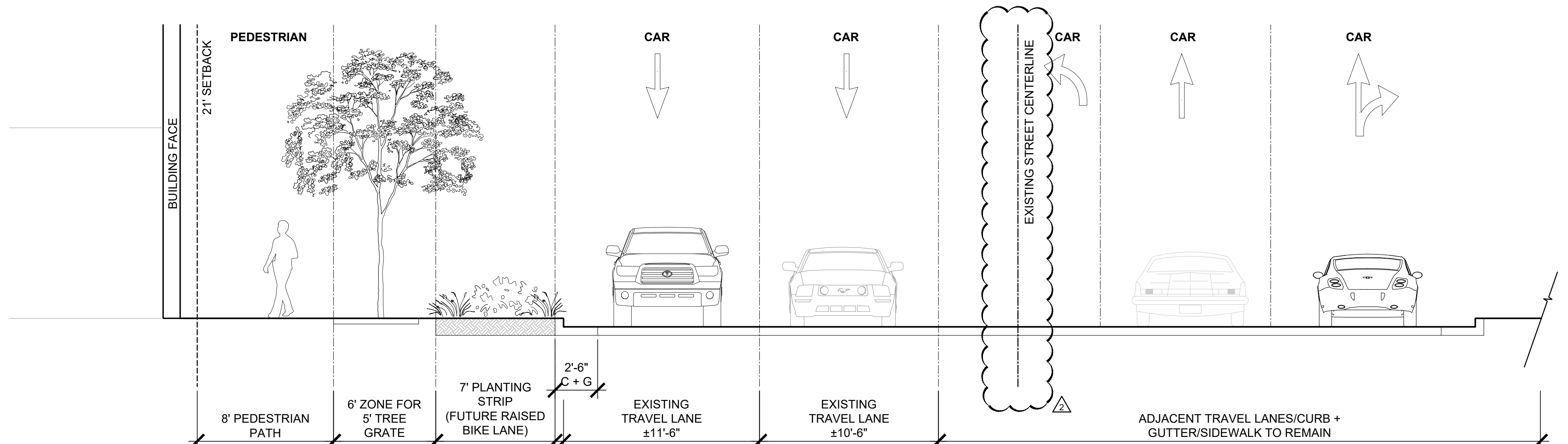
SECTION A - SOUTH TRYON STREET SCALE: 1/4" = 1'-0"
