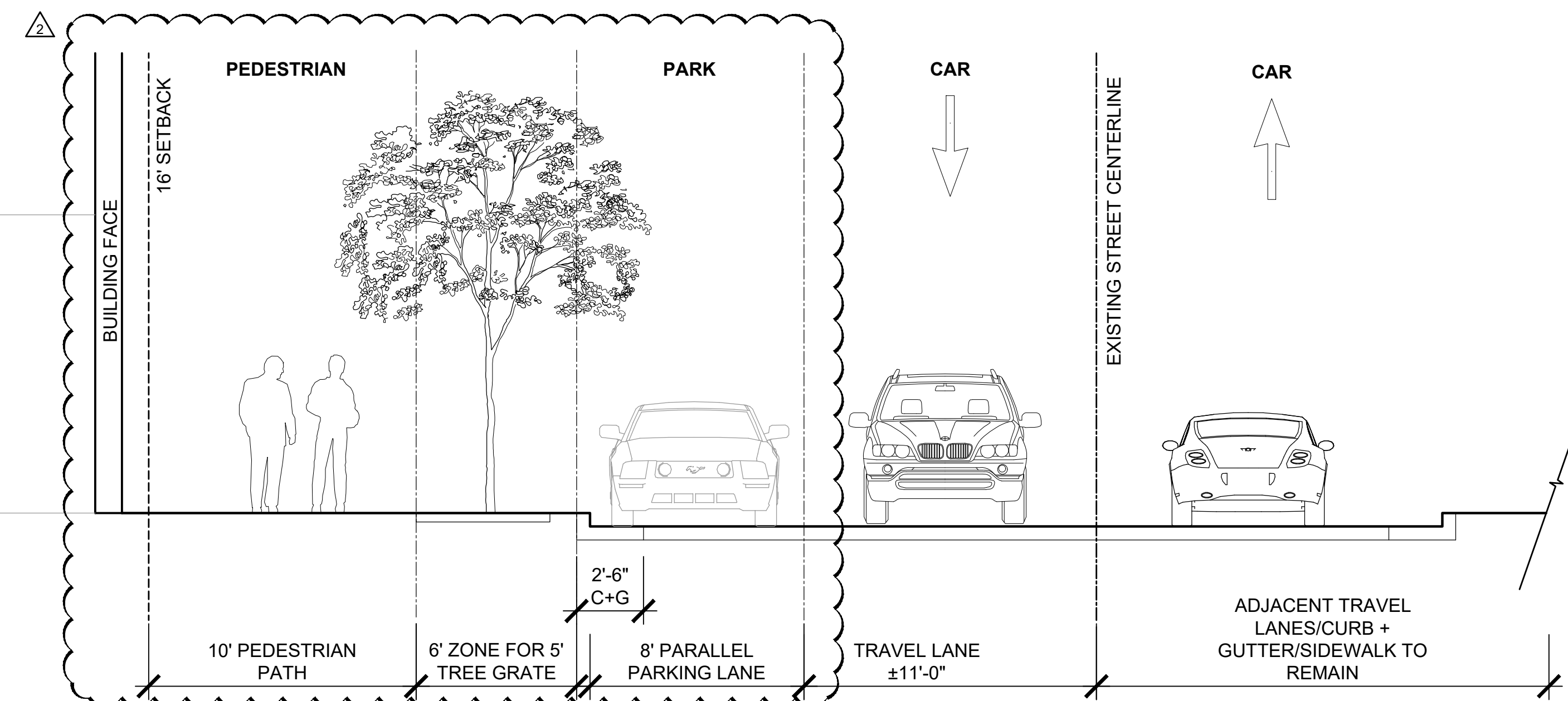
SECTION C - HAWKINS STREET SCALE: 1/4" = 1'-0"
