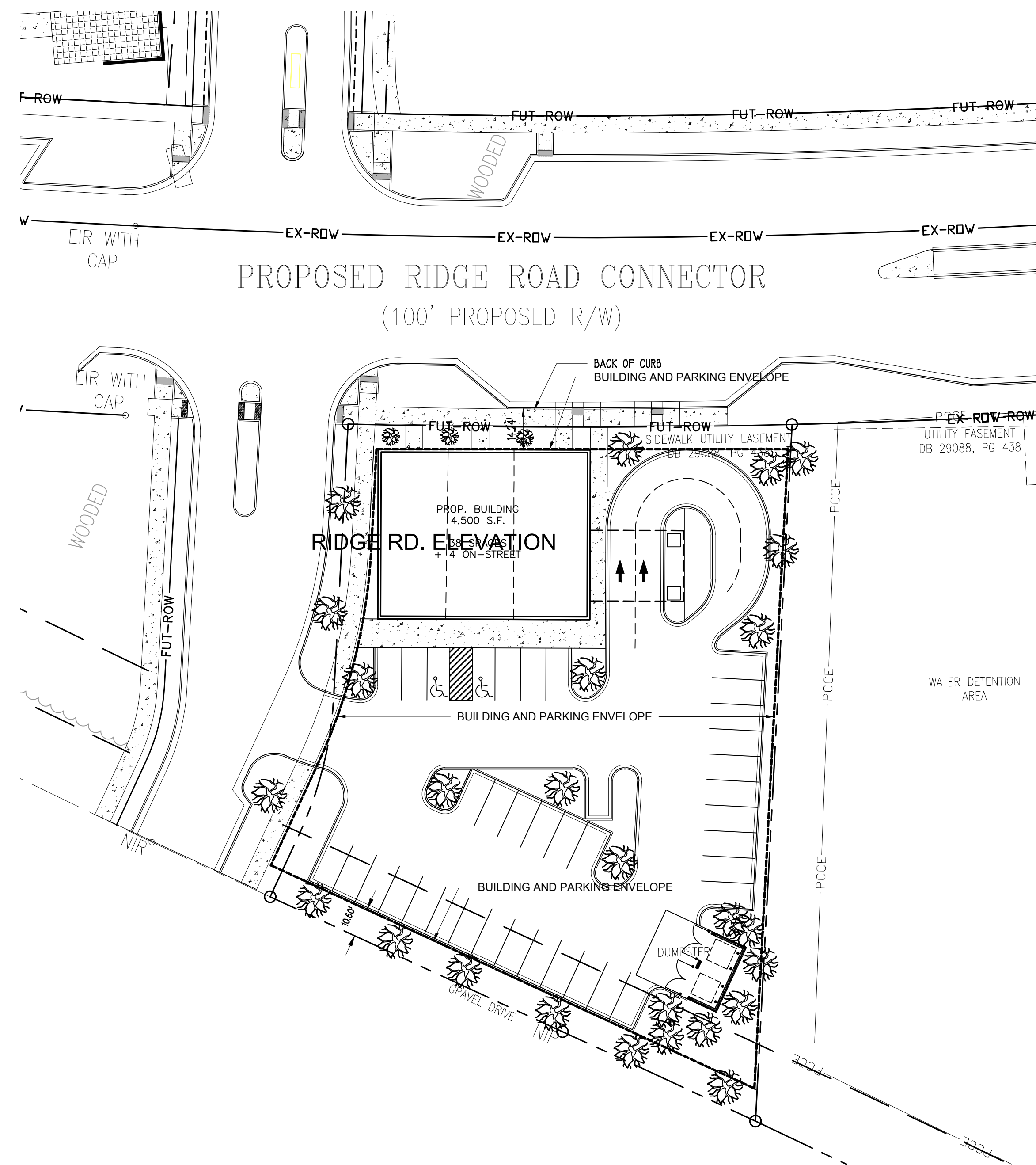
1 SITE PLAN 1"=30.0'
