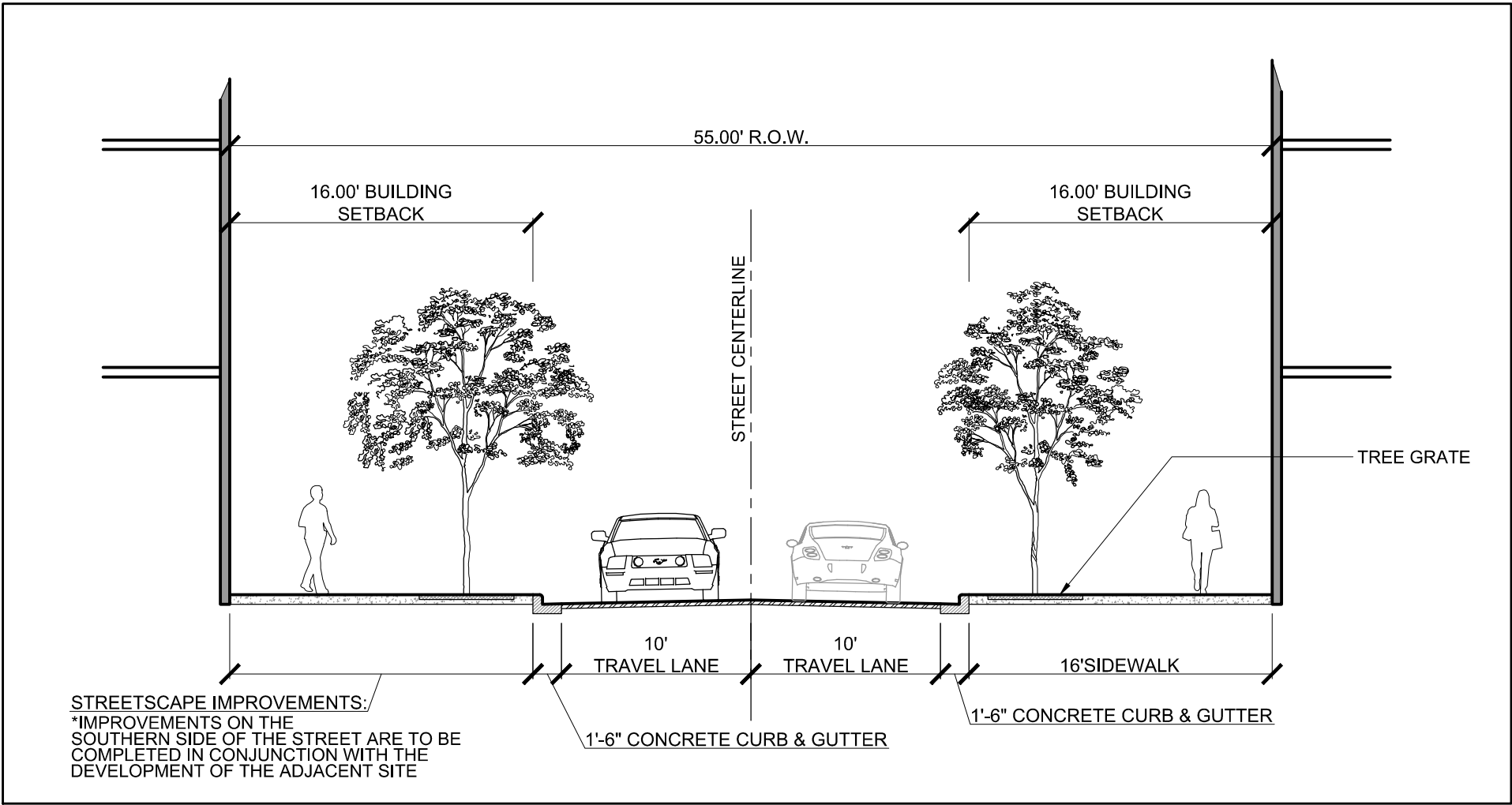
35TH STREET CROSS SECTION
