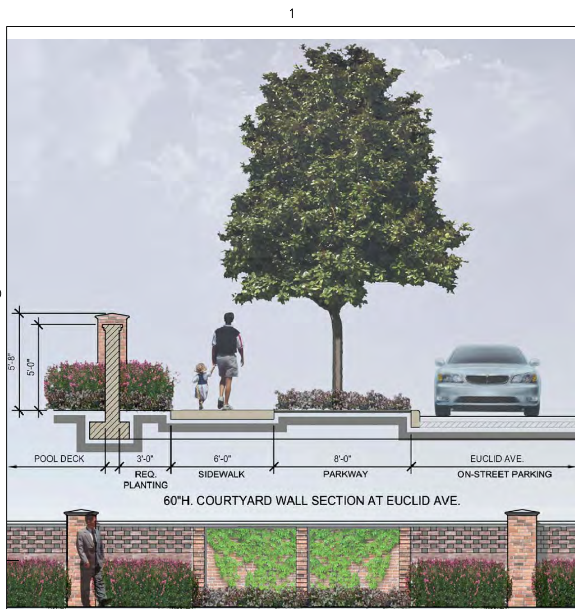
D3 POOL WALL DETAIL NTS
