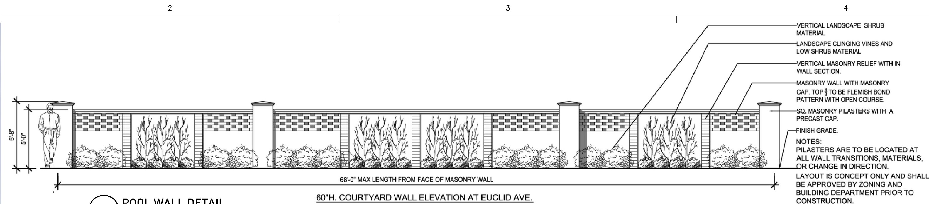
D2 POOL WALL DETAIL NTS
