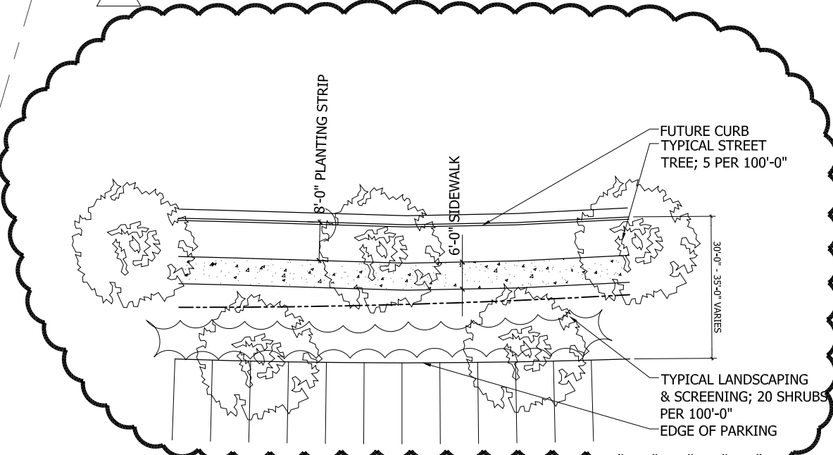
02 TYP. 100' SECTION HARRIS BLVD.
