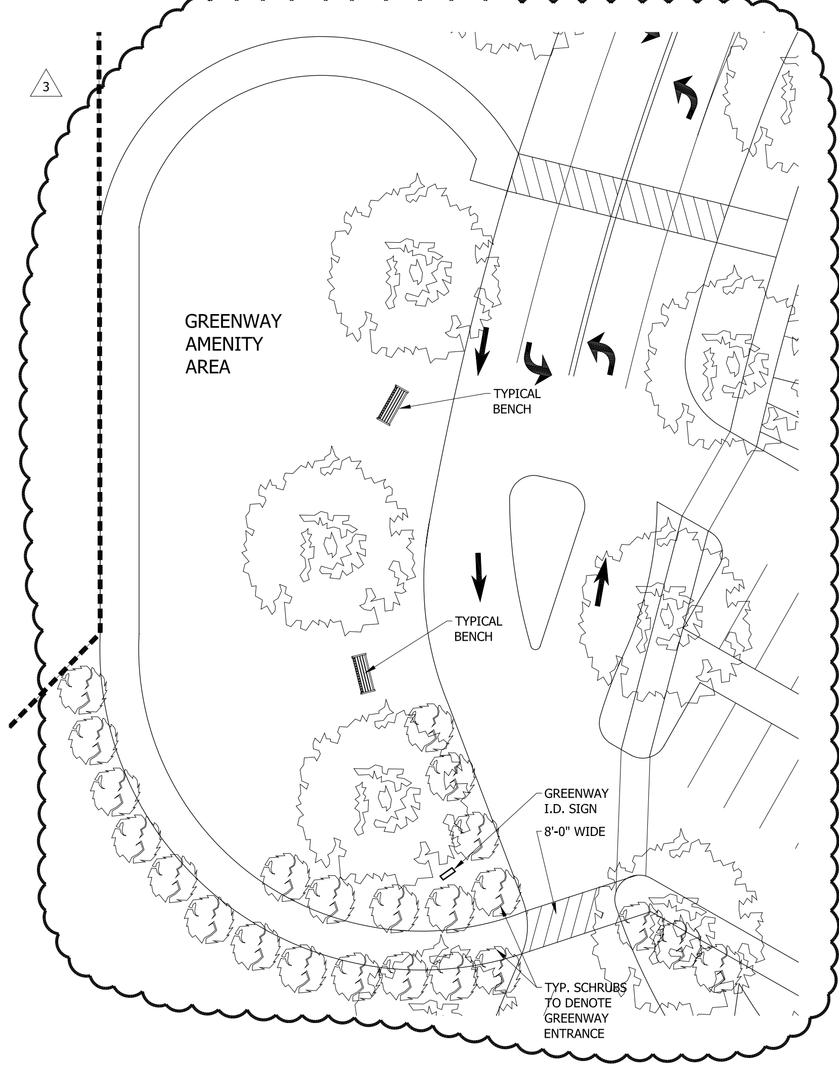
03 ILLUSTRATIVE PLAN - GREENWAY AMENITY AREA 1"=20'-0"
