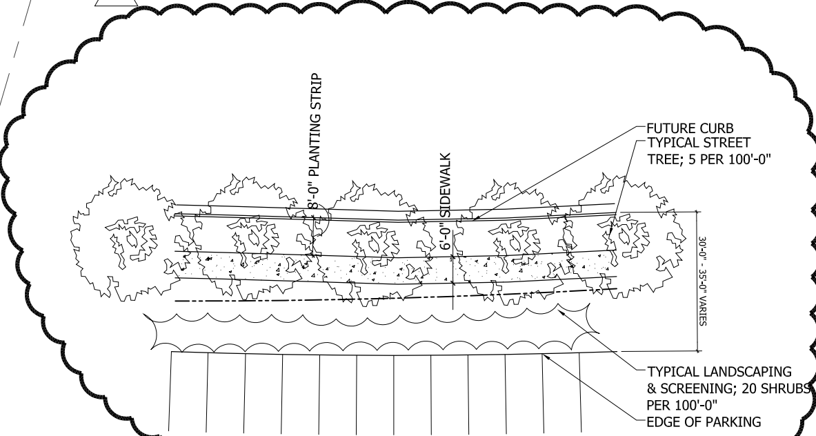
02 TYP. 100' SECTION HARRIS BLVD.
