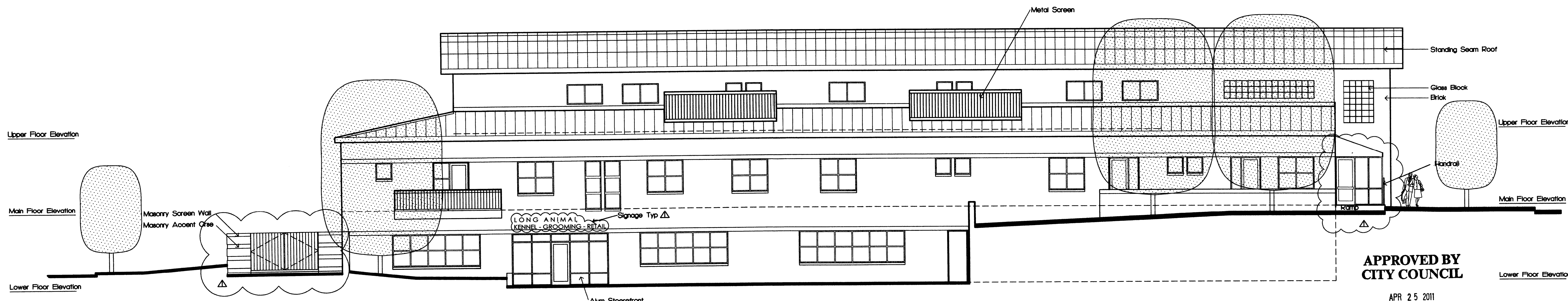
North Elevation
