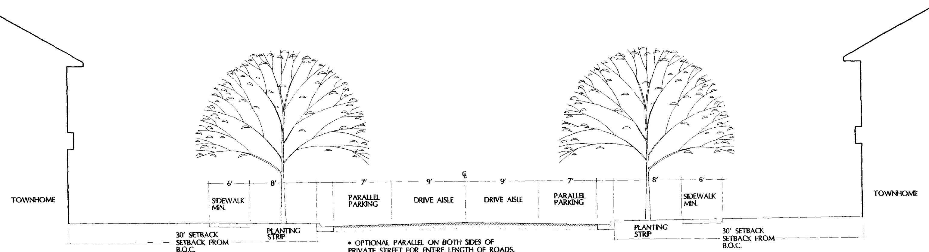
PRIVATE STREET SECTION
