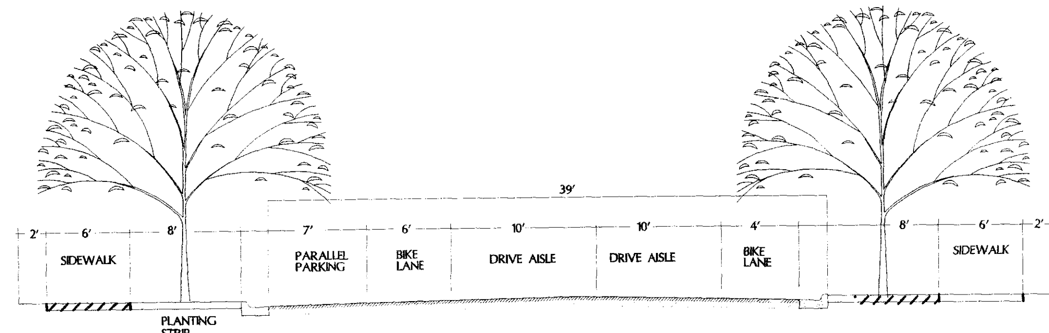
Proposed Thoroughfare Section NTS
