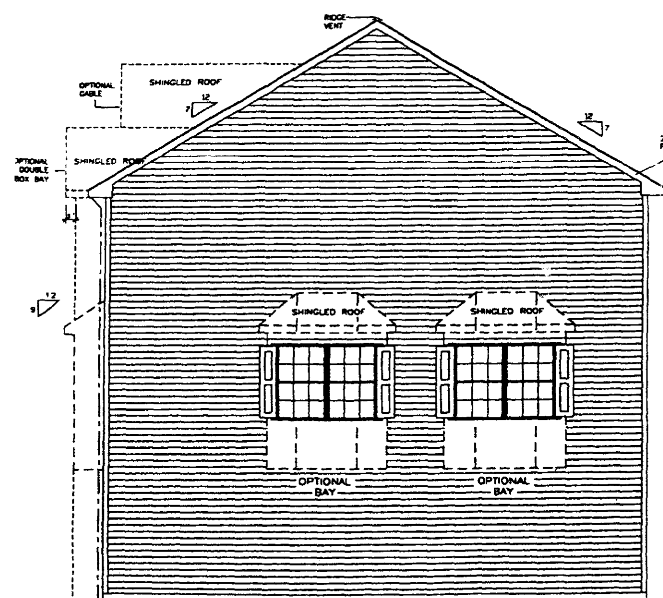
END UNIT ELEVATION Kitchen Front Condition
